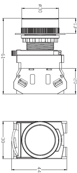
Flat pushbutton
