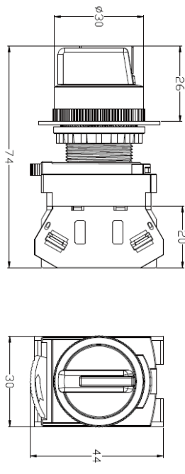
Selector 3 position
