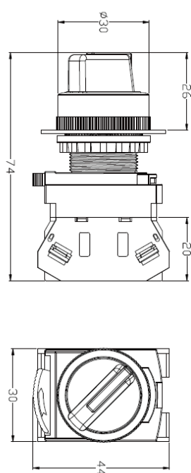
Selector 2 position
