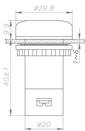
Compact indicator
