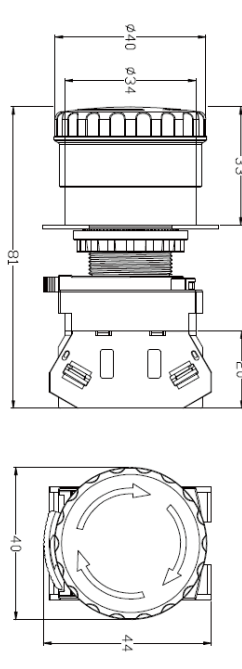
Emergency pushbutton
