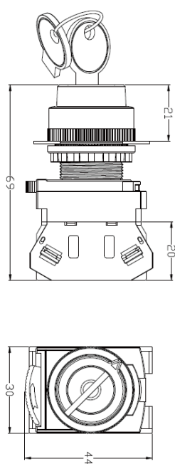
Key-operator 2 positions
