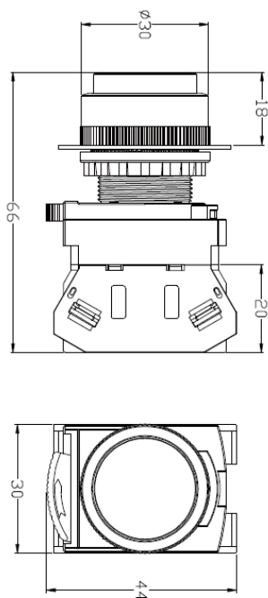
Extend pushbutton
