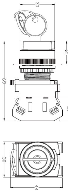
Key-operator 3 positions
